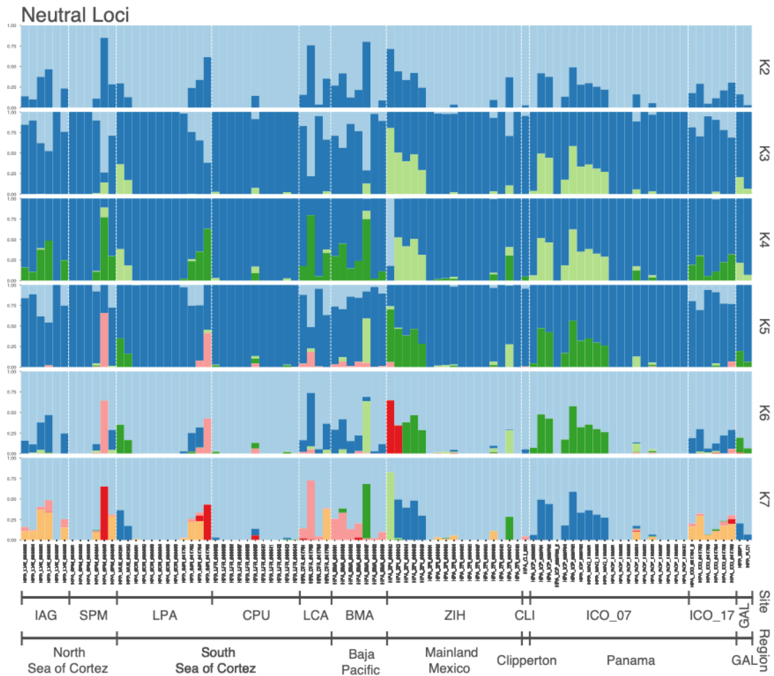
Figure S2. STRUCTURE plots generated from 19,635 neutral loci for H. passer for K=2-7 . The most likely number of clusters based on \Delta K was K=3 . Sampling sites and regions are arranged from North to South and from West to East of the TEP. Sampling site key: IAG- Isla Ángel de la Guarda, SPM- San Pedro Mar, LPA- La Paz, CPU- Cabo Pulmo, LCA- Los Cabos, BMA- Bahía Magdalena, ZIH- Zihuatanejo, CLI- Clipperton, ICO_07- Isla Contadora 2007, ICO_17- Isla Contadora 2017, GAL- Galapagos.
