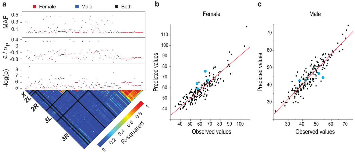
Fig. 4. Genotype-phenotype associations for starvation resistance. (a) GWA results for significant SNPs. The lower triangle depicts LD ( r^2 ) among SNPs, with the five major chromosome arms demarcated by black lines. The upper panels give the significance threshold ( -\log_{10}p , uncorrected for multiple tests), the effect in phenotypic standard deviation units, and the minor allele frequency (MAF). (b-c) Partial Least Squares regressions of phenotypes predicted using SNP data on observed phenotypes. The blue dots represent the predicted and observed phenotypes of lines that were not included in the initial study. (b) Females ( r^2 = 0.81 ). (c) Males ( r^2 = 0.85 ).
