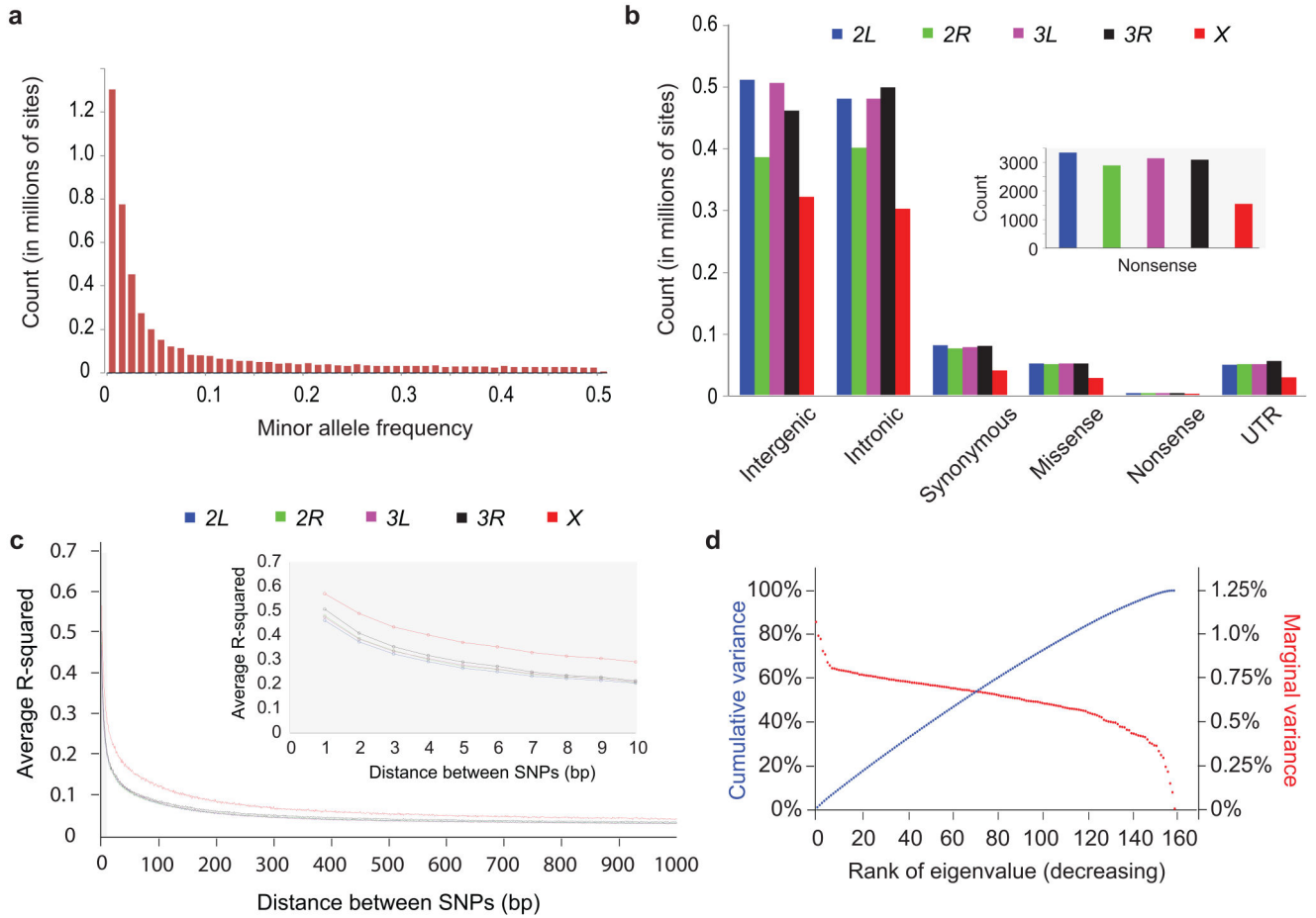
Fig. 1. SNP variation in the DGRP lines. (a) Site frequency spectrum. (b) Numbers of SNPs per site class. (c) Decay of LD ( r^2 ) with physical distance for the five major chromosome arms. (d) Lack of population structure. The red curve depicts the ranked eigenvalues of the genetic covariance matrix in decreasing order with respect to the marginal variance explained; the blue curve shows their cumulative sum as a fraction of the total with respect to cumulative variance explained. The partitioning of total genetic variance is balanced among the eigenvectors. The principal eigenvector explains <1.1% of the total genetic variance.
