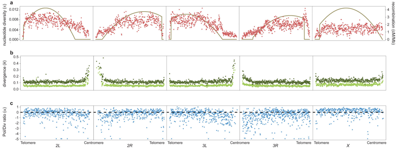
Fig. 2. Pattern of polymorphism, divergence, \alpha and recombination rate along chromosome arms in non-overlapping 50 kbp windows. (a) Nucleotide polymorphism ( \pi ). The solid curves give the recombination rate (cM/Mb). (b) Divergence ( k ) for D. simulans (light green) and D. yakuba (dark green). (c) Polymorphism/Divergence, estimated as 1 - [(\pi_{0\text{-fold}}/\pi_{4\text{-fold}})/(k_{0\text{-fold}}/k_{4\text{-fold}})] . An excess of 0-fold divergence relative to polymorphism ( k_{0\text{-fold}}/k_{4\text{-fold}} > (\pi_{0\text{-fold}}/\pi_{4\text{-fold}}) ) is interpreted as adaptive fixation while an excess of 0-fold polymorphism relative to divergence ( \pi_{0\text{-fold}}/\pi_{4\text{-fold}} > (k_{0\text{-fold}}/k_{4\text{-fold}}) ) indicates weakly deleterious or nearly neutral mutations are segregating in the population. Tel: telomere; Cent: centromere.
