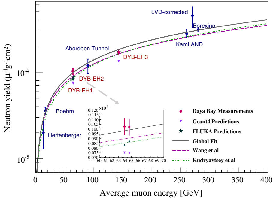
FIG. 13. Neutron yield vs. average muon energy from the three Daya Bay experimental halls compared to other experiments. The points for Daya Bay EH1 and EH2, which differ in energy by less than 1 GeV, are shown in the inset. The predicted yields at Daya Bay from GEANT4 and FLUKA are also shown. Experimental data is shown from Hertenberger [6], Boehm [8], Aberdeen Tunnel [10], KamLAND [4], LVD [2] with corrections from [35], and Borexino [3]. The solid line shows the power-law fit to the global data set including Daya Bay. The dashed line and dash-dotted lines show FLUKA-based predictions for the dependence of the neutron yield on muon energy from Wang et al. [32] and Kudryavtsey et al. [33].
