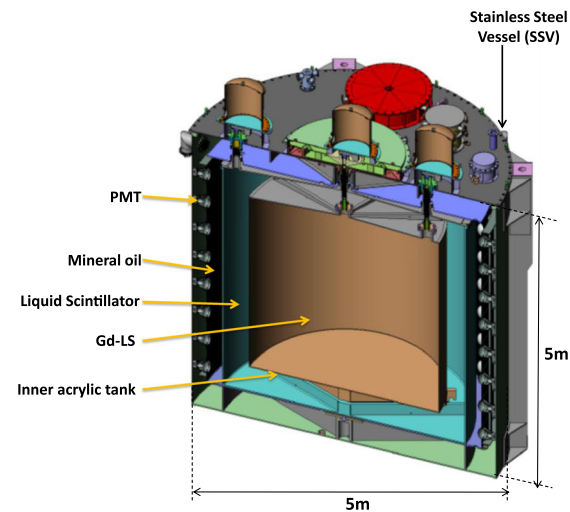
FIG. 2. Left: Diagram of near site detectors. Right: Diagram of an AD.
