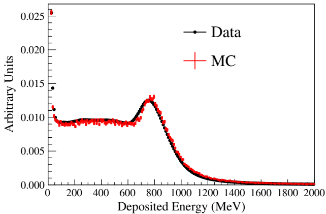
FIG. 6. Distribution of energy deposited in an AD by AD-tagged muons that fall within a [-2 \mu\text{s}, 2 \mu\text{s}] time window of a water-pool tagged muon in data and MC (EH1). For data, the deposited energy is reconstructed from PMT hits. For MC, the simulated deposited energy is shown.
