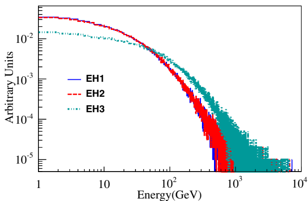
FIG. 5. Simulated energy spectra of muons that reach the underground halls. The differences between EH1 and EH2 are too small to be visible at this scale.
