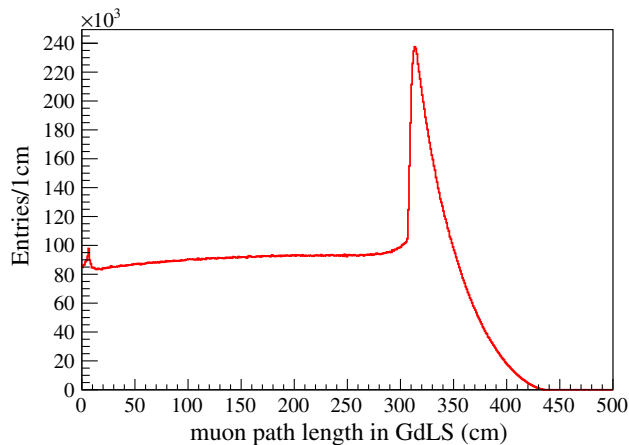
FIG. 7. Distribution of muon path length through the GdLS from simulation (EH1). The small peak at \sim 6.5 cm is due to the geometry of the calibration tubes in the AD. The large peak around 300 cm corresponds to the dimensions of the of the GdLS region.
