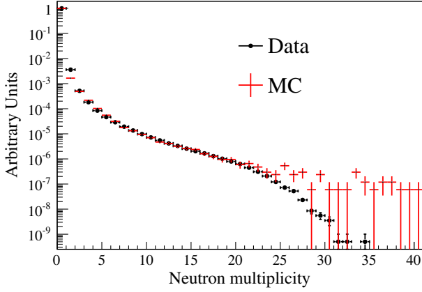
FIG. 9. Comparison of neutron multiplicity in data and MC in EH1. For the MC, true neutron captures on Gd are selected between 10 and 200 \mu\text{s} after an AD-tagged muon. For the data, neutron captures are selected with a 6–12 MeV energy range between 10 and 200 \mu\text{s} after an AD-tagged muon. To suppress random background in the data, no other AD-tagged muon is allowed in a [-0.5, 0.5] ms window. This distribution has been corrected for readout window efficiency and the effect of blocked triggers.
