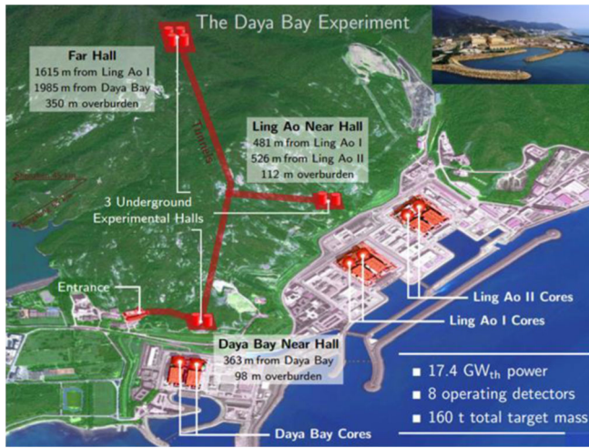
FIG. 1. A map of the layout of the Daya Bay Reactor Neutrino Experiment, including six reactor cores (Daya Bay, Ling Ao I, and Ling Ao II cores) and three experimental halls (two near and one far). The antineutrino detectors (ADs) are located in the underground experimental halls, with two ADs at the Daya Bay Near Hall (EH1), two at the Ling Ao Near Hall (EH2), and four at the Far Hall (EH3).
