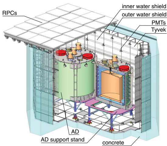
FIG. 2. Left: Diagram of near site detectors. Right: Diagram of an AD.
