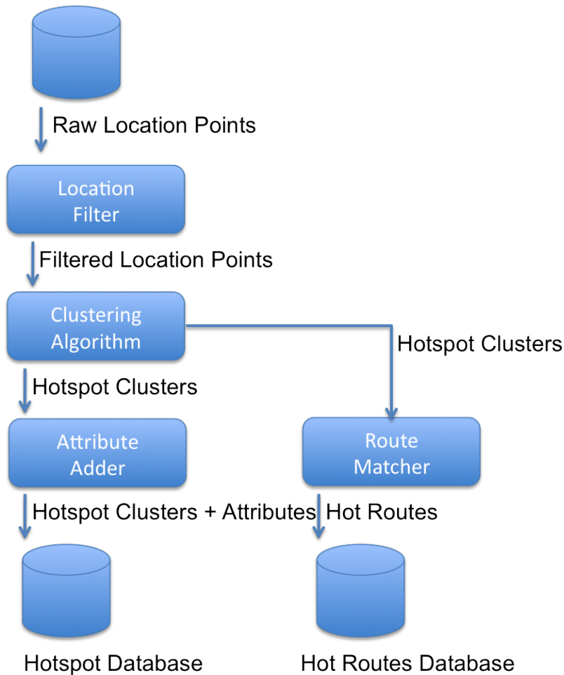
Figure 17: Hotspot algorithm flowchart
