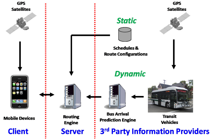
Figure 1: Architecture and system implementation of BayTripper.
