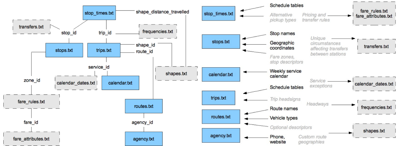
Figure 7: GTFS file structure. Optional Files in dashed boxes, Required files in solid boxes (a) Files and linking columns (b) Properties of files needed to be extracted
