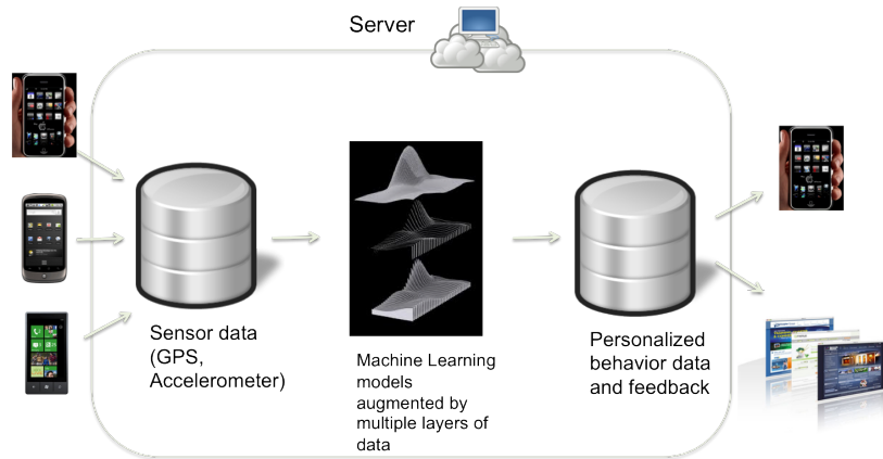
Figure 22: System Architecture Diagram. The components of the system consist of mobile phones, trip determination algorithms running on a server, and web tools to view and correct trips.
