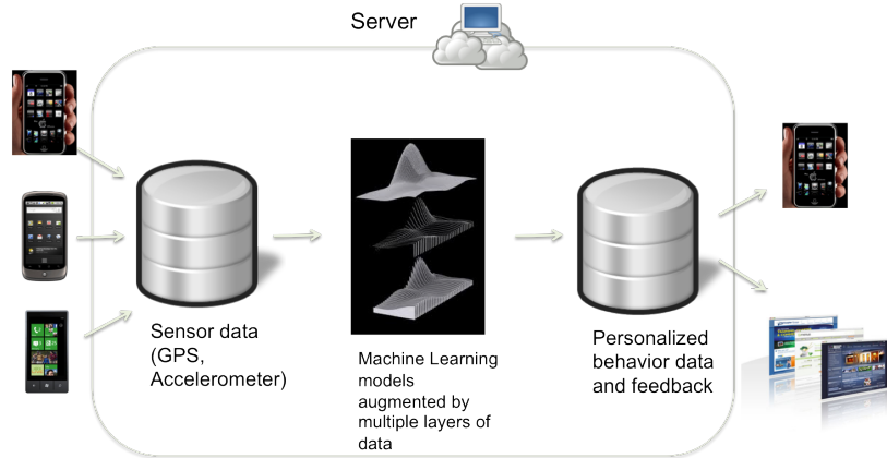
Figure 13: System Architecture Diagram. The components of the system consist of mobile phones, trip determination algorithms running on a server, and web tools to view and correct trips.
