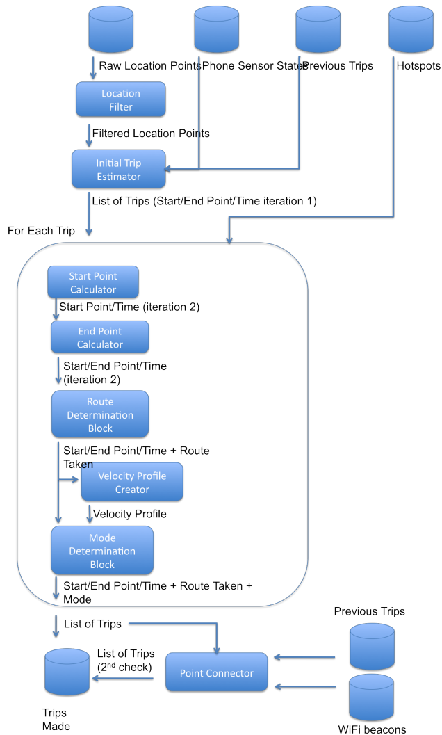
Figure 16: Overall algorithm flowchart. Each block and data source is described in Sections 4.4.1 - 4.4.9
