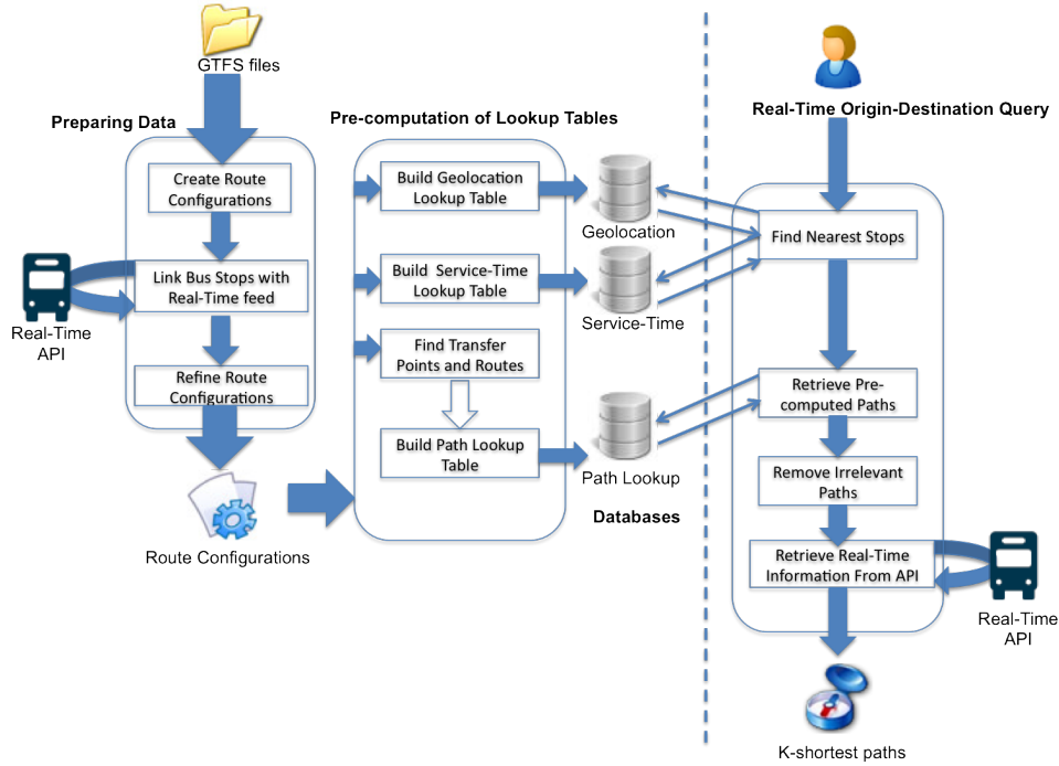
Figure 5: Flowchart of the algorithm described in Sections 3.2.1, 3.2.5, and 3.2.10.
