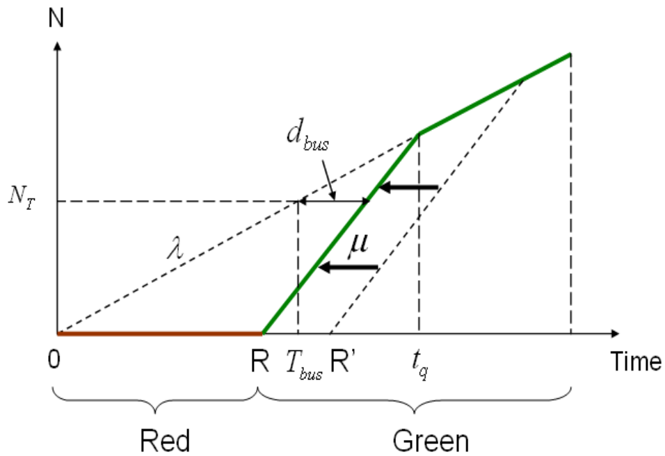
Figure 4-6 N-T curve for bus movement with TSP
