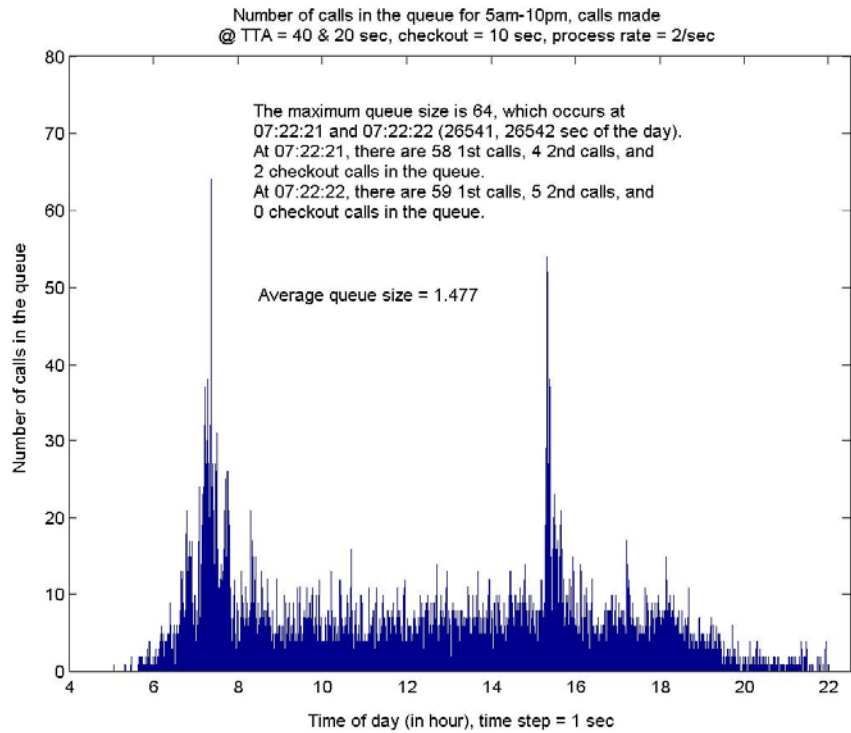
Figure 7-19 Number of calls in the queue; multiple requests {40, 20, 10}
