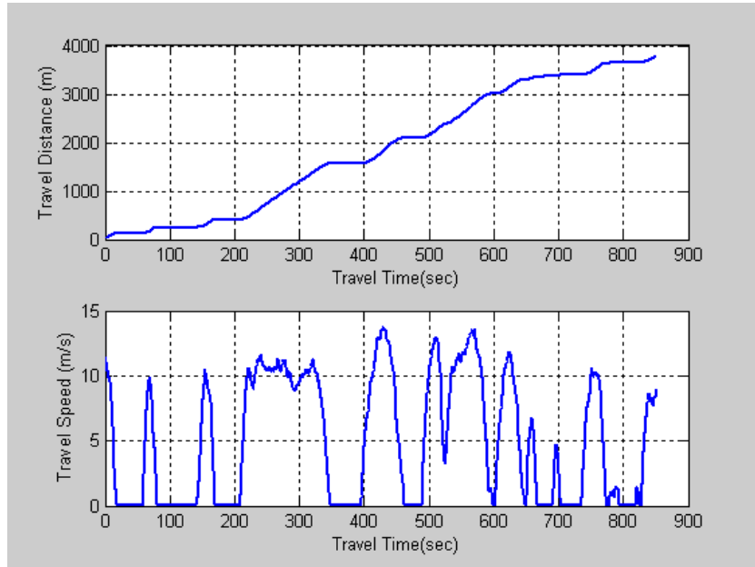
Figure 2-1 Bus Location and Speed as Function of Time
