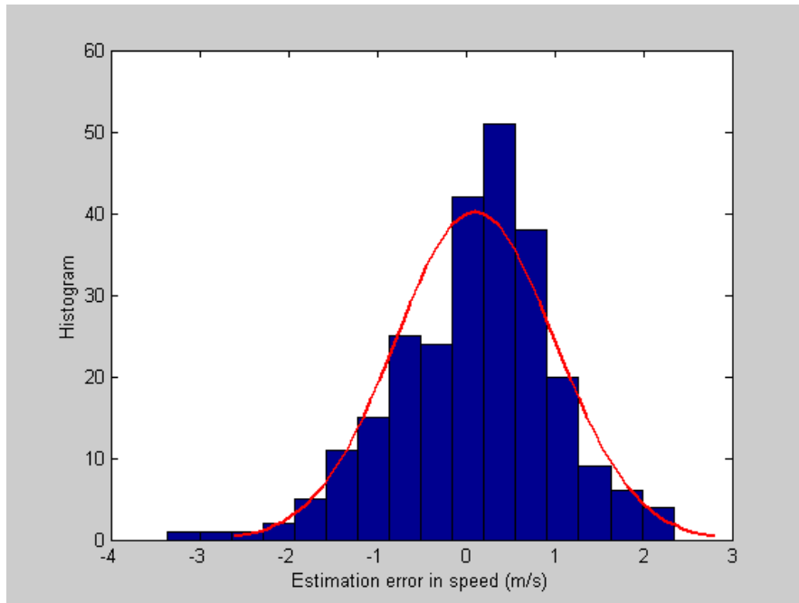
Figure 2-6 Histogram of Speed Estimation Error by Equation 2-23
