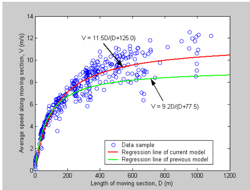
Figure 2-3 Regression Lines of Equation 2-3 and Equation 2-23
