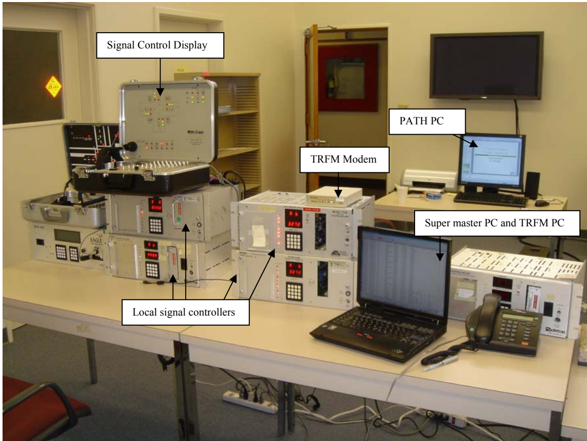
Figure 5-3 Hardware-in-the-loop Simulation Test-bed
