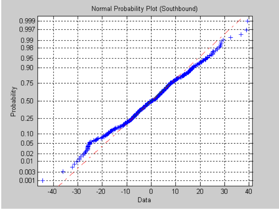
Figure 3-4 Normal Probability Plot for Southbound Increment
