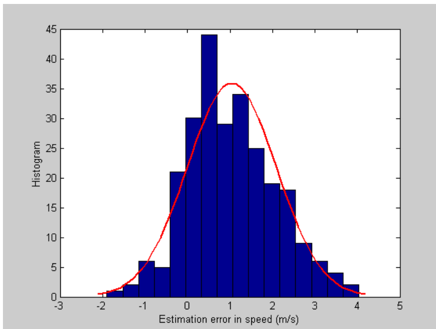
Figure 2-7 Histogram of Speed Estimation Error by Equation 2-3
