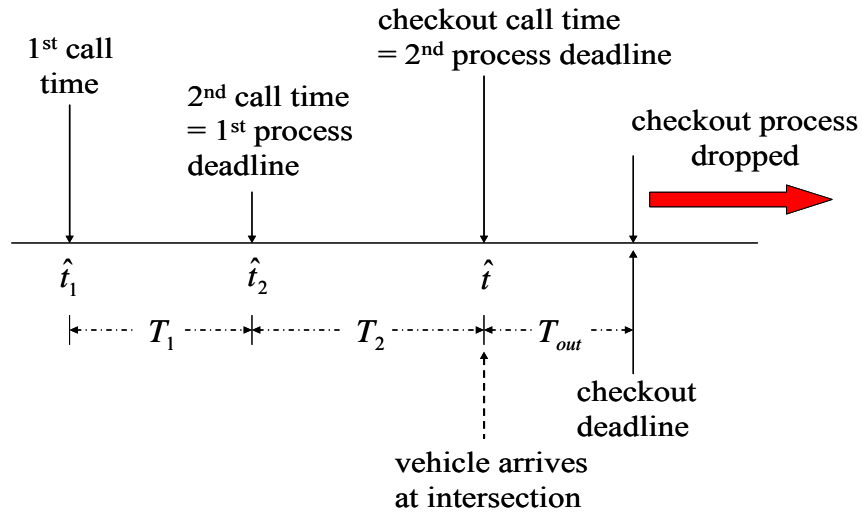
Figure 7-15 Timelines of multiple priority request processes
