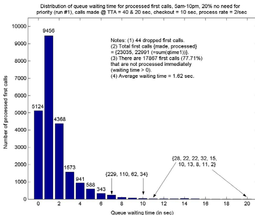
Figure 7-29 Histogram of first call waiting time; 20% no need for priority
