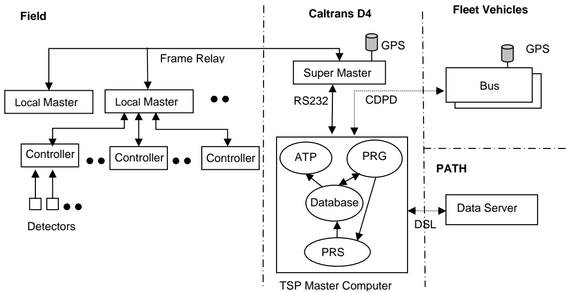
Figure 1-1 System Architecture of the Prototype ATSP System
