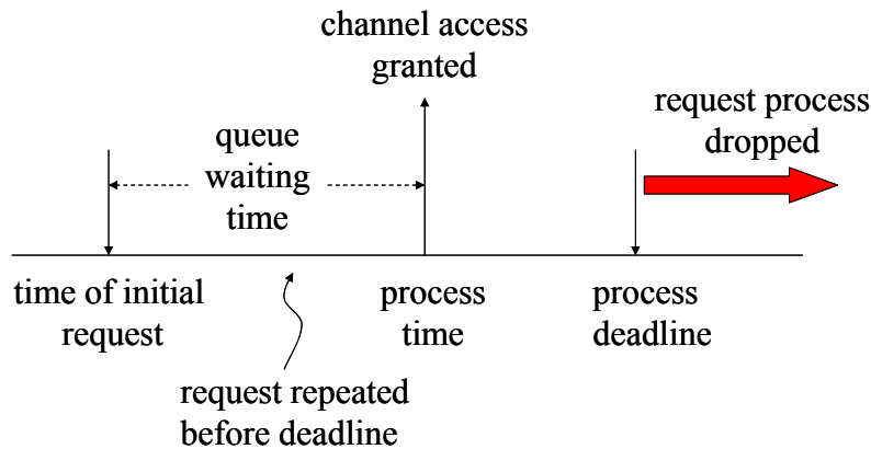
Figure 7-10 Timeline of a single priority request process
