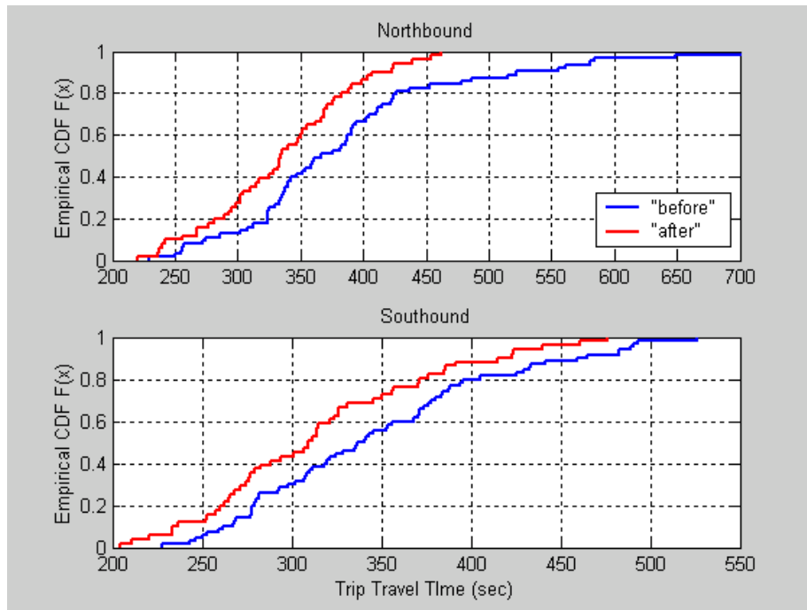
Figure 6-2 CDF Plot of Bus Trip Travel Time
