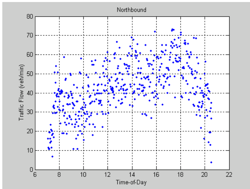
Figure 3-1 Traffic Flow v.s. Time-of-Day (Northbound)
