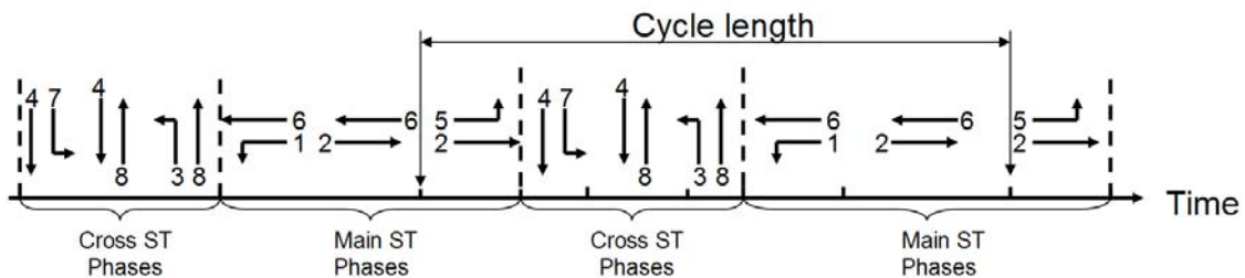
Figure 4-4 Expanded phase sequence for the example
