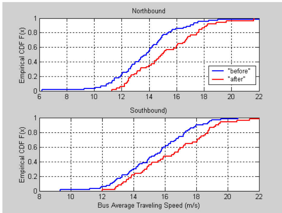
Figure 6-3 CDF Plot of Bus Average Traveling Speed
