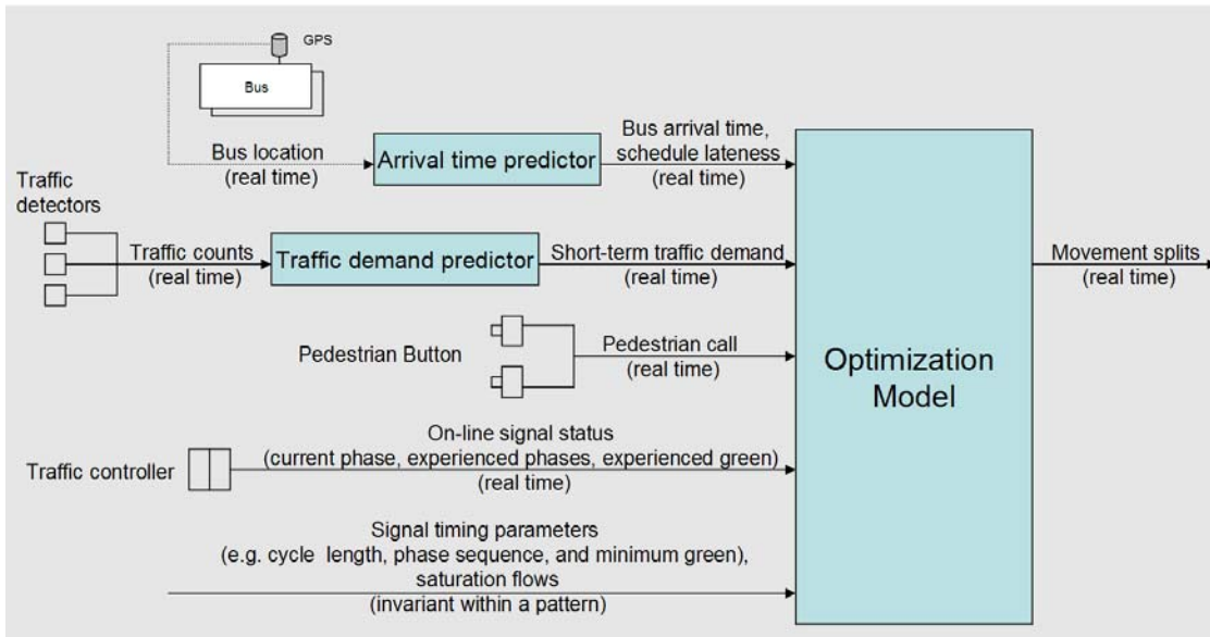
Figure 4-2 Control input/output diagram
