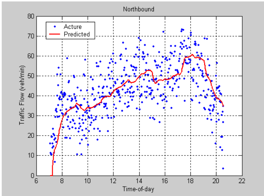
Figure 3-1 Predicted Traffic Flow (Northbound)
