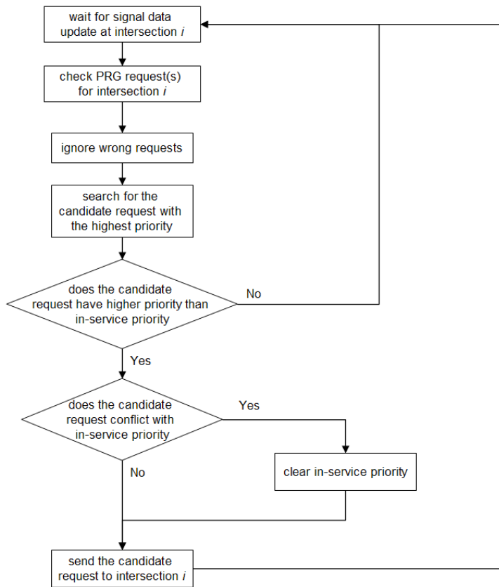
Figure 1-2 Flow Chart of TSP Algorithm
