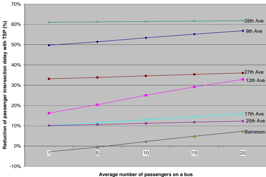
Figure 6-5 Sensitivity analysis of passenger delay reduction (%)
