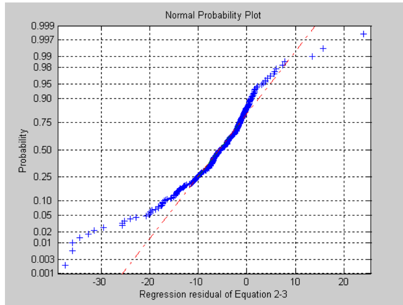
Figure 2-5 Normal Probability Plot of Regression Residual of Equation 2-3
