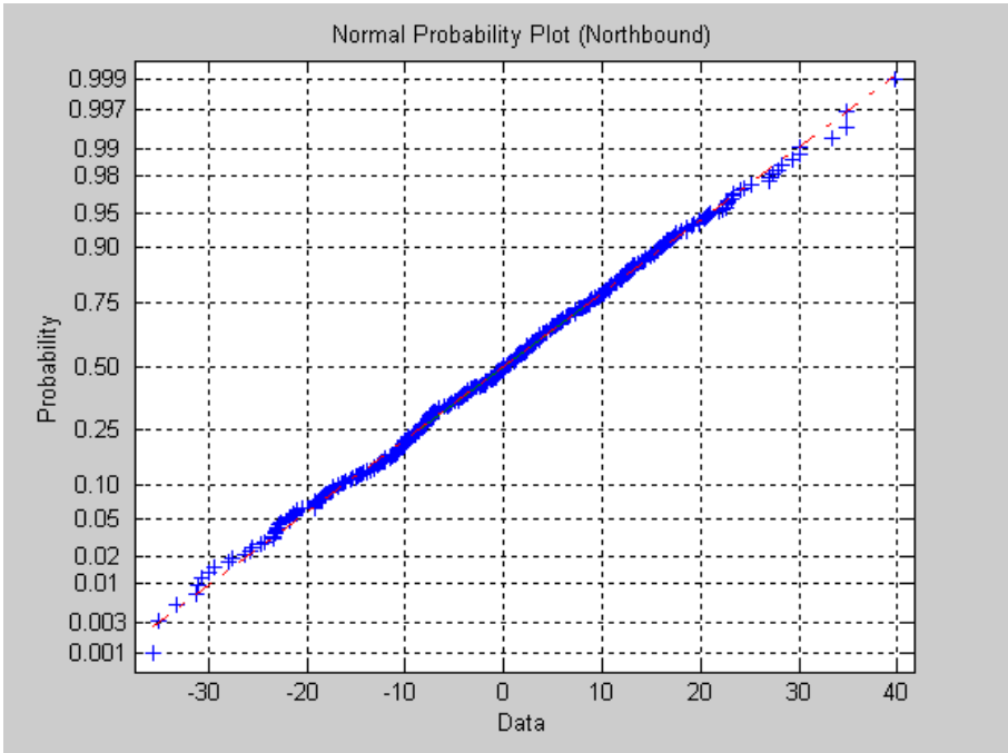
Figure 3-3 Normal Probability Plot for Northbound Increment
