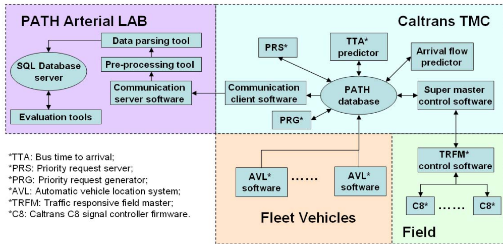
Figure 5-2 ATSP System Software Architecture
