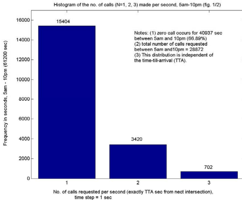
Figure 7-8 Histogram of the number of simultaneous calls for 5am-10pm (part 1/2)
