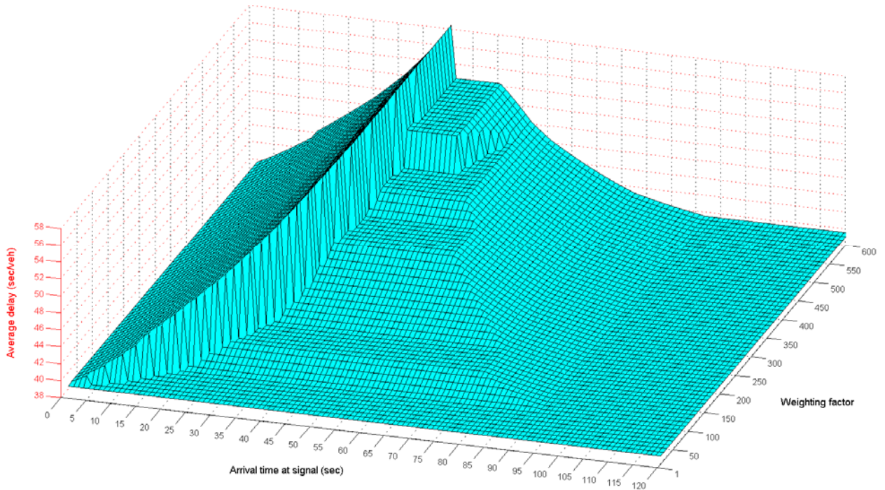
Figure 4-8 Intersection delay for other traffic in the heavily congested scenario
