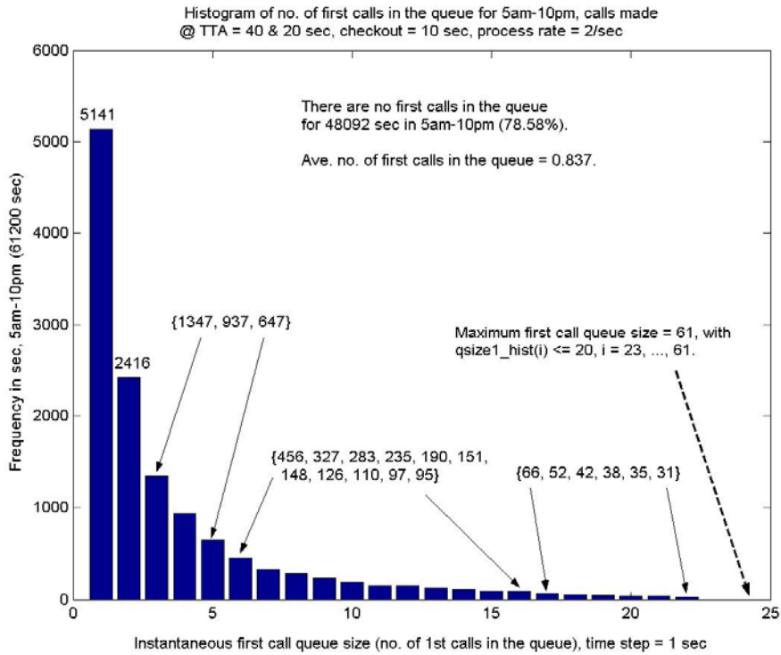
Figure 7-22 Histogram of first call queue size; multiple requests {40, 20, 10}
