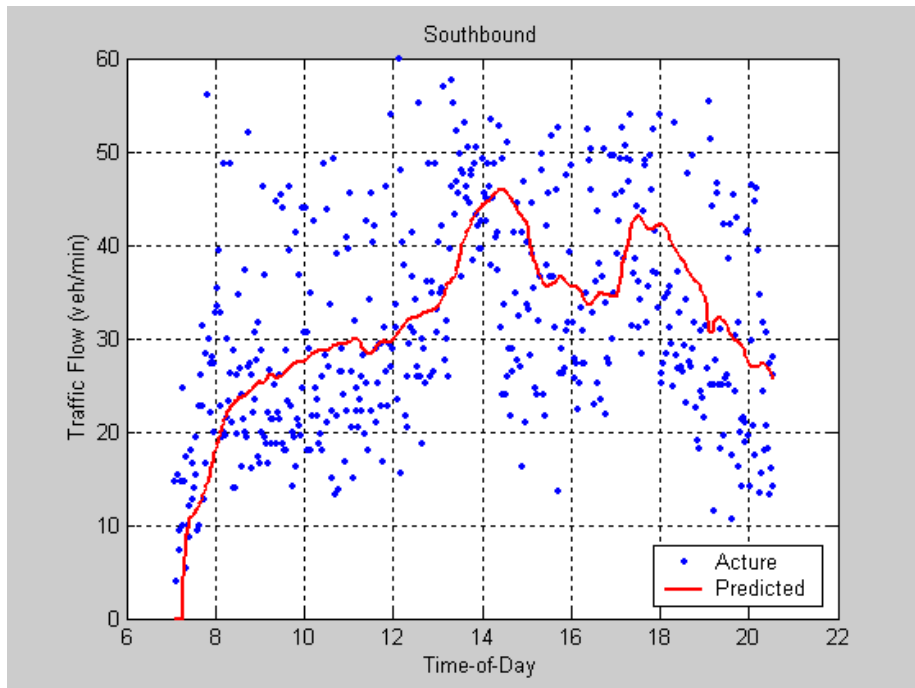
Figure 3-2 Predicted Traffic Flow (Southbound)
