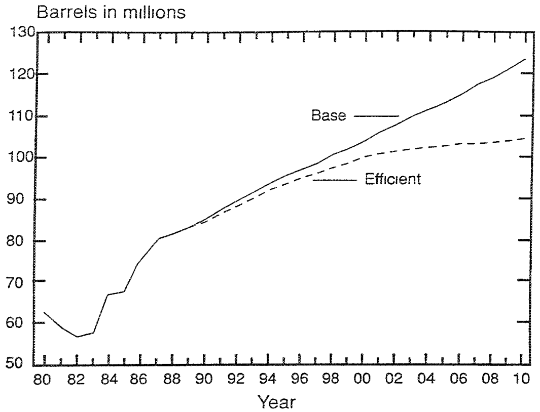
FIGURE 2-6 California Annual Jet Fuel Consumption Forecast.
