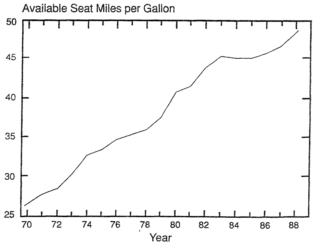
FIGURE 2-5 U.S. Jet Fleet Fuel Efficiency.
