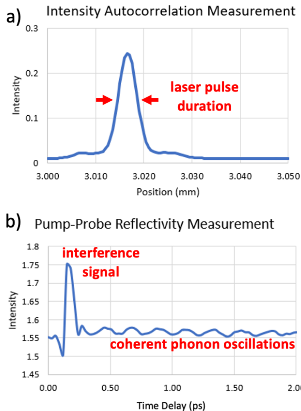
Figure 5. a) An example of the data obtained from an intensity autocorrelation measurement. The peak is the intensity autocorrelation signal, which is fit with a Gaussian for the students to determine the temporal width of the laser pulses. b) An example of the pump-probe reflectivity data obtained with the single-crystalline antimony sample. The peak near the beginning of the measurement is caused by the interference of the simultaneous pump and probe beams on the sample surface. The less-intense oscillations that continue to the end of the scan window are the coherent a_{1g} phonon oscillations obtained through the reflectivity changes of the probe pulse versus time. The period of oscillation is fit by the students with sine functions and converted to a value in units of frequency.
