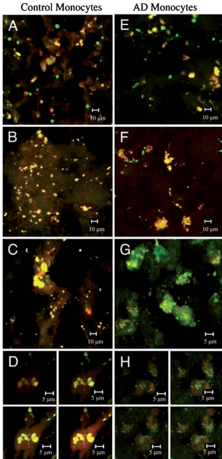
Fig. 2. Uploading of A \beta (red) from AD brain tissue after incubation for 2 days and 4 days with normal and AD monocytes (green). Note that normal monocytes bind to neurons and up load A \beta (become golden); AD monocytes also bind to neurons but up load A \beta poorly and shrivel into apoptosis (from Fiala et al. [2]).
