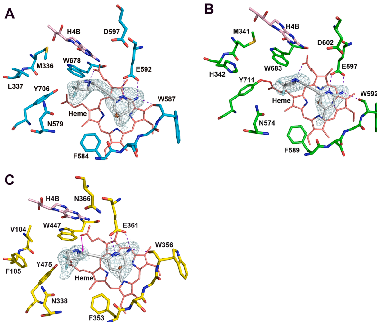
Fig. 7. Active site structures of 17 bound to rnNOS (A), hnNOS (B), and heNOS (C). A clash (pink arrow) was observed between the alkyne linker and propionate A in heNOS.
