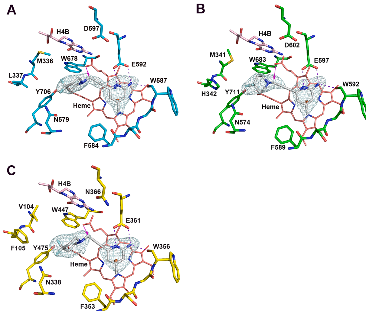
Fig. 8. Active site structures of 19 bound to mNOS (A), hnNOS (B), and heNOS (C). In all three cases, the clashes of the alkyne linker with propionate A were present (pink arrows).
