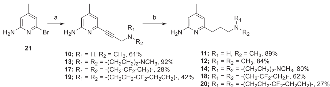
Scheme 1. General synthetic approaches to compounds 10–14 and 17–20 . (a) The appropriate propargyl amine, Pd(PPh 3 ) 4 (5 mol%), PPh 3 (10 mol%), CuI (10 mol%), Et 3 N, 120 °C, CH 3 CN (0.23 M), 24 h, 28–93%; (b) Pd/C or Pd(OH) 2 /C (10–40 mol%), H 2 , CH 3 OH, 25–80 °C, 8–24 h, 27–89%.
