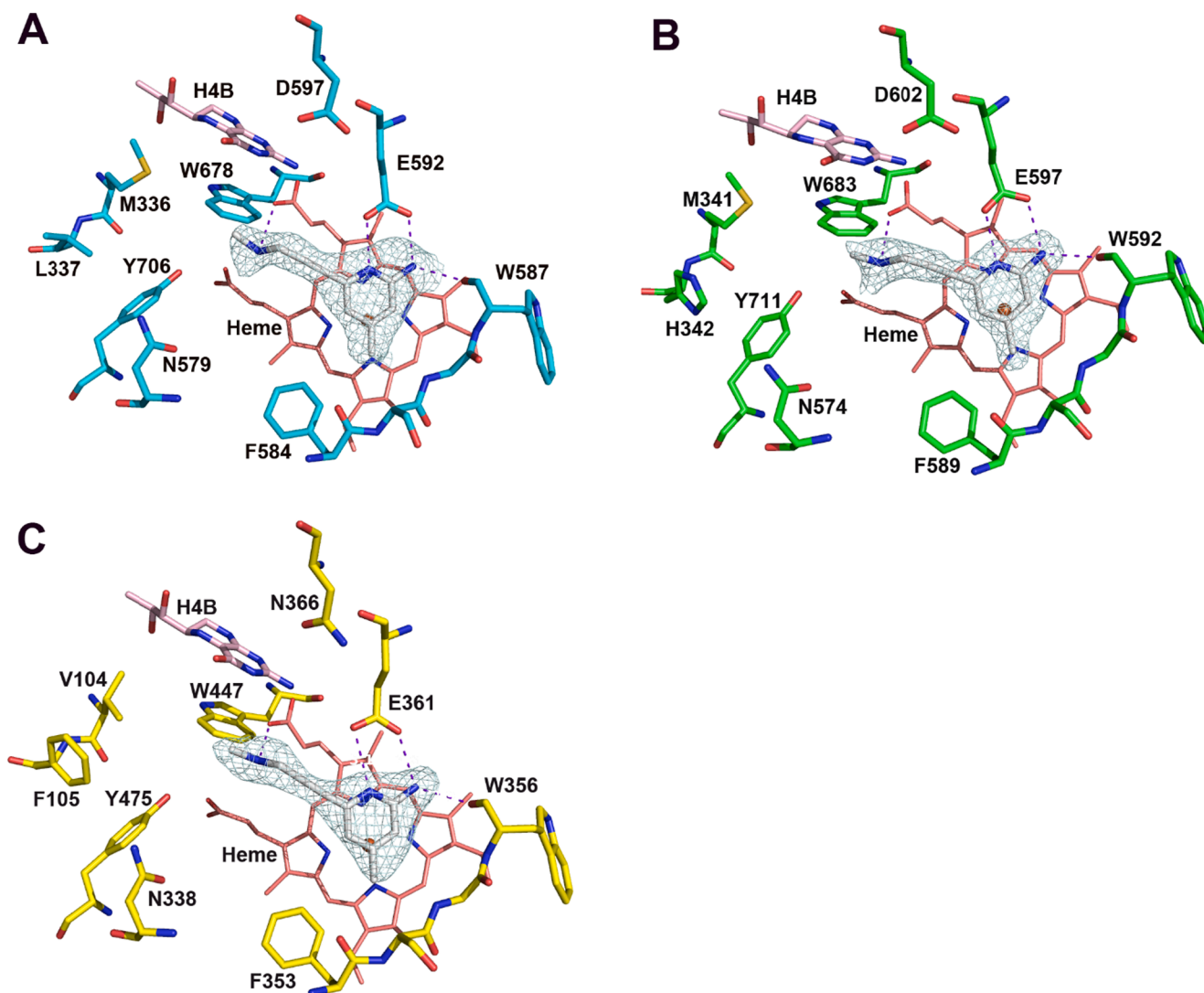
Fig. 5. Active site structures of 10 bound to rNOS (A), hnNOS (B), and heNOS (C).
