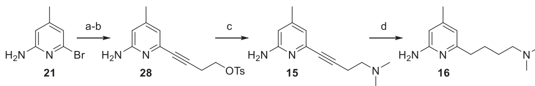
Scheme 3. Synthesis of compounds 15–16. (a) But-3-yn-1-ol, Pd(PPh 3 ) 4 (5 mol%), CuI (10 mol%), Et 3 N, 120 °C, CH 3 CN (0.25 M), 18 h, 70%; (b) TsCl, DMAP, Et 3 N, DCM, 0 °C to 25 °C, 17 h, 53%; (c) (CH 3 ) 2 NH, K 2 CO 3 , CH 3 CN, 80 °C, 9 h, 68%; (d) Pd/C (10%), H 2 , CH 3 OH, 25 °C, 24 h, 62%.
