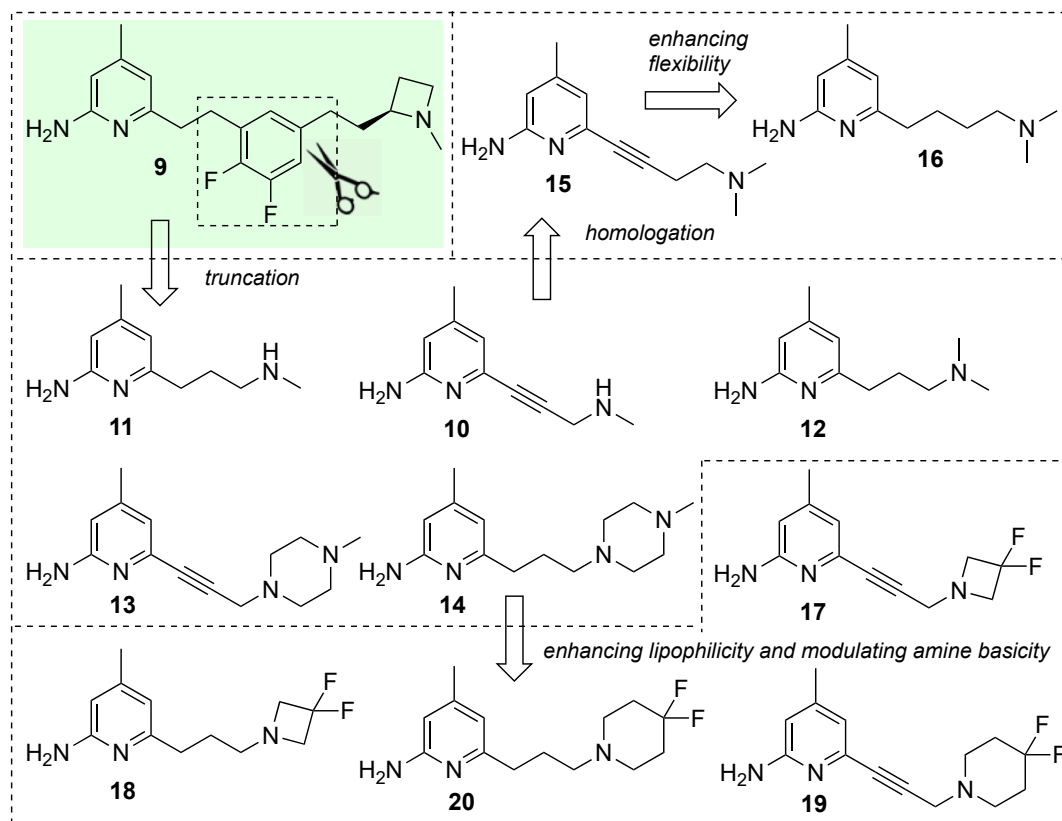
Fig. 2. Analogues from lead 9 with a reduced number of rotatable bonds.
