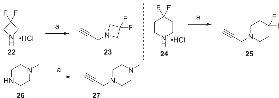
Scheme 2. Synthesis of propargyl amines 23 , 25 and 27 . (a) propargyl bromide, K 2 CO 3 , CH 3 CN, 25 °C, 8 h, 48–53%.
