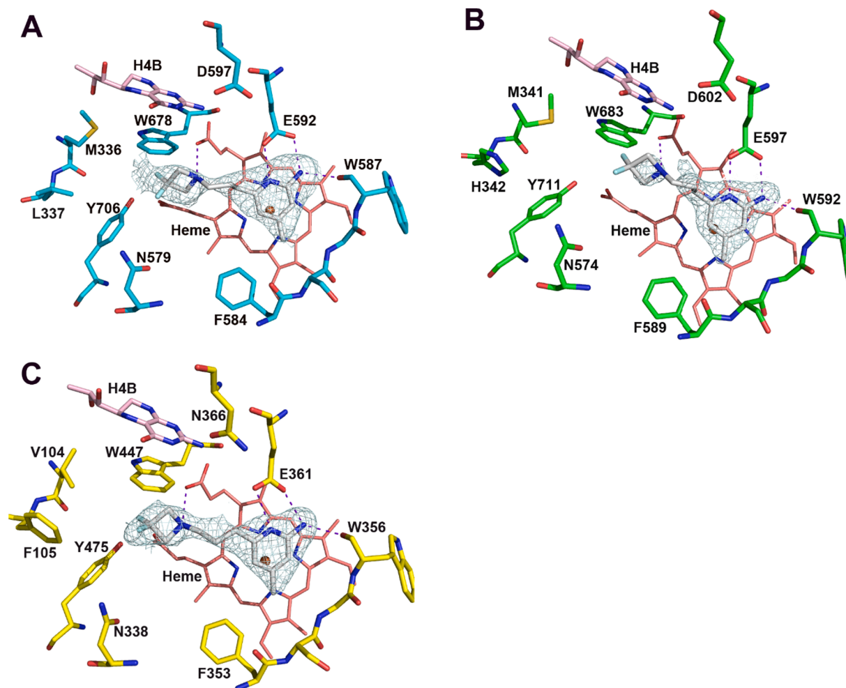
Fig. 9. Active site structures of 18 bound to mNOS (A), hnNOS (B), and heNOS (C).
