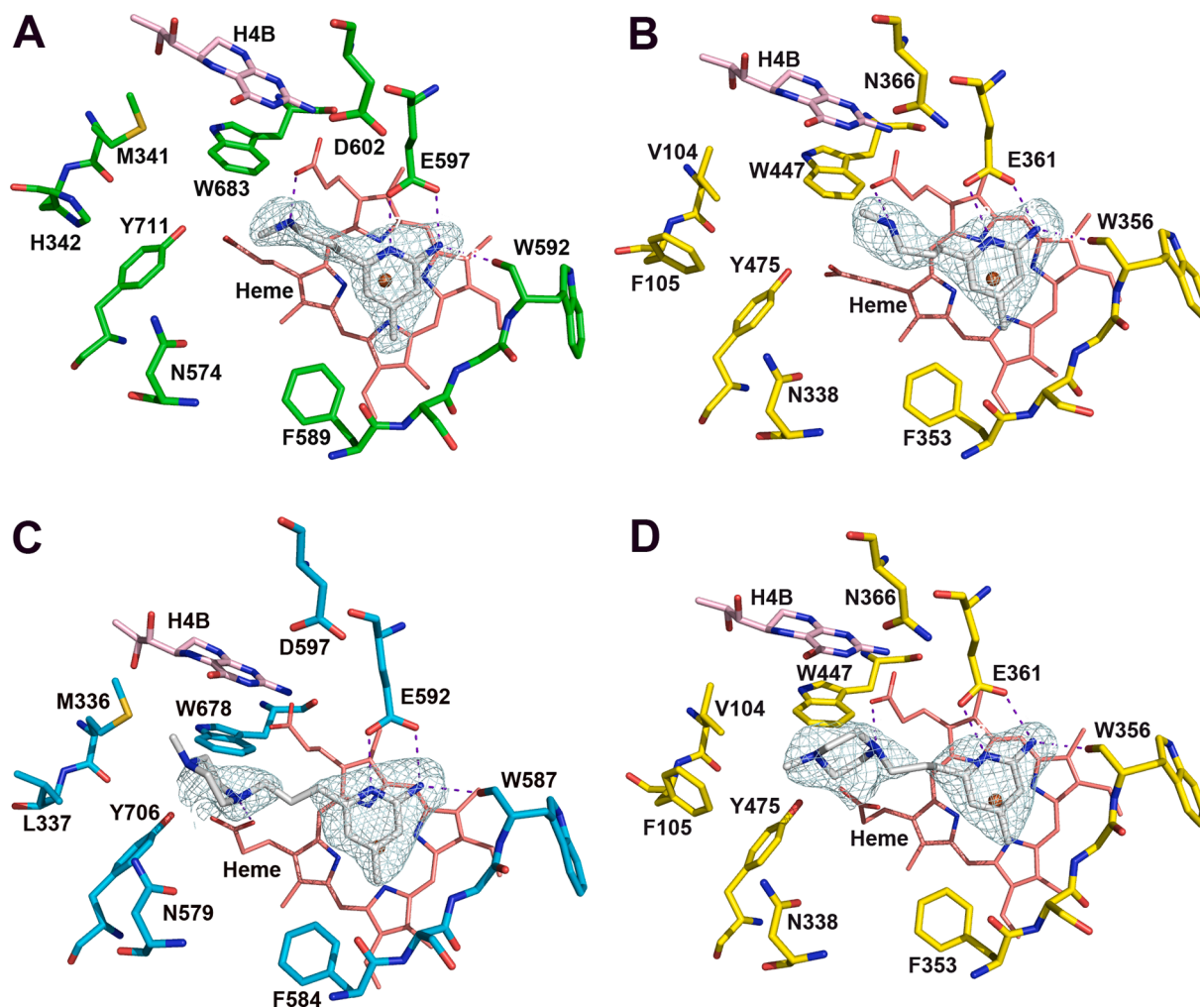
Fig. 4. Active site structures of 11 bound to hnNOS (A) and heNOS (B); and 14 bound to rnNOS (C) and heNOS (D).
