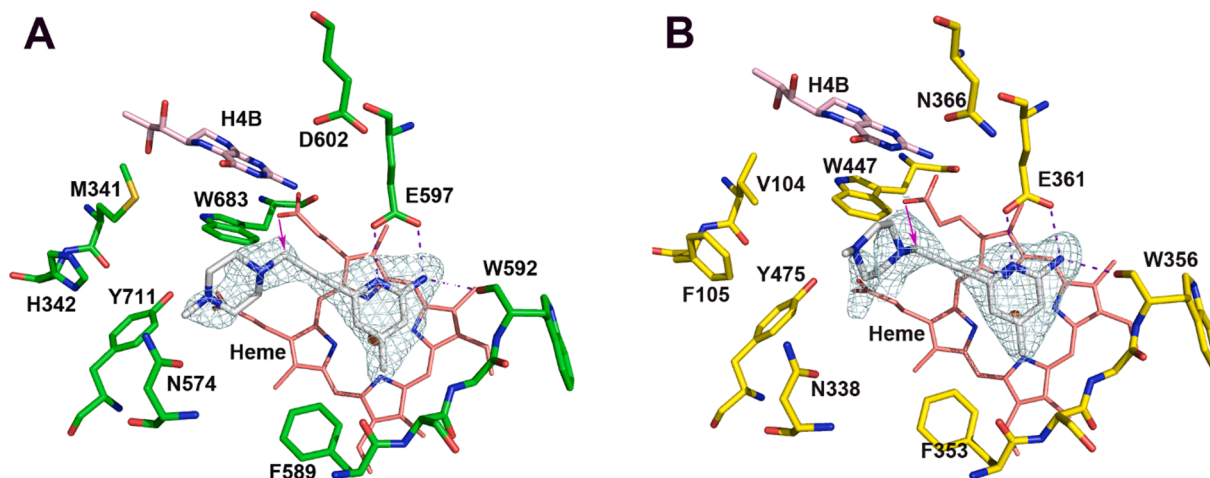
Fig. 6. Active site structures of 13 bound to hnNOS (A) and heNOS (B). The clashes observed between the rigid alkyne linker and propionate A are shown by the pink arrows.
