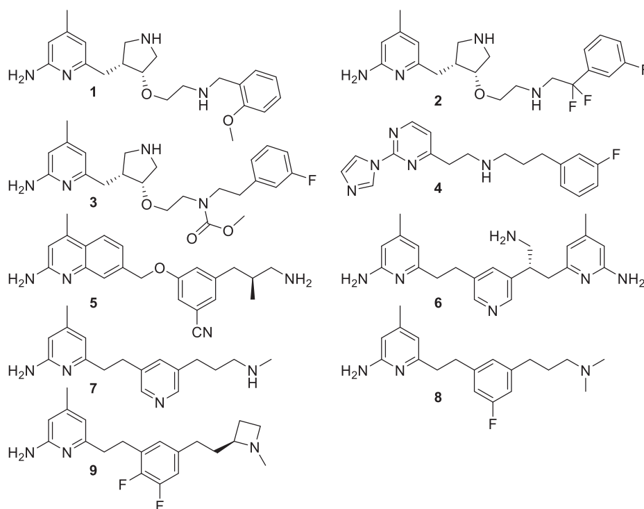
Fig. 1. Structure of recent nNOS inhibitors.
