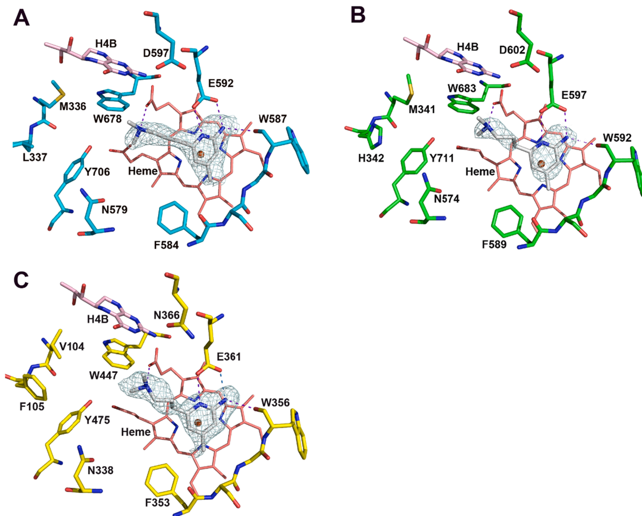
Fig. 3. Active site structures of 12 bound to rNOS (A), hnNOS (B), and heNOS (C). In all structural figures, the following atomic color schemes are used: cyan, green, and yellow for carbon atoms in the rNOS, hnNOS, and heNOS backbones, respectively; red, oxygen; blue, nitrogen; light cyan, fluorine. The omit F o -F c Polder electron density for the inhibitor is shown at the 3.0 \sigma contour level. Key H-bonds to the inhibitor are depicted with dashed lines.
