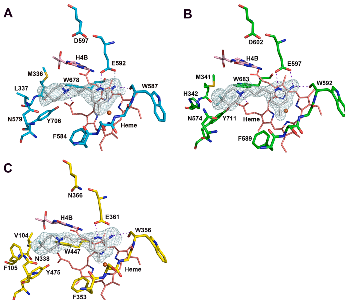
Fig. 10. Active site structures of 20 bound to rNOS (A), hnNOS (B), and heNOS (C).
