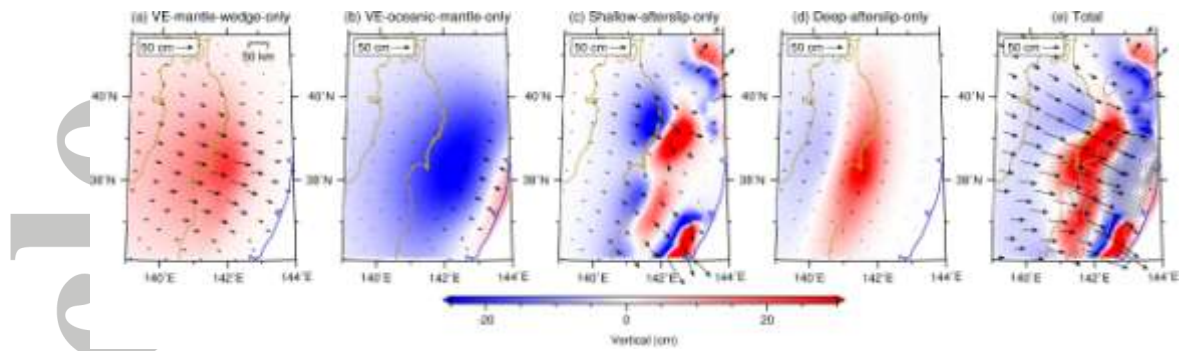
Figure 4. Separated contributions of relaxation in the rheological elements to the modeled surface deformation. Viscosities of the rheological elements are the same as that in the LAM (Figure 6b). Black arrows and contours represent cumulative two-year horizontal and vertical postseismic displacements, respectively. Solid brown lines represent coast lines. Gray contours in (e) represent coseismic slip contours of the 2011 earthquake ( Iinuma et al. , 2012). (a) Surface deformation only due to the viscoelastic relaxation of the continental upper mantle and no afterslip in the shear zone. The oceanic upper mantle is assumed to be elastic in this test. (b) Surface deformation only due to the viscoelastic relaxation of the oceanic upper mantle and no afterslip in the shear zone. The continental upper mantle is elastic. (c) Surface deformation only due to the afterslip in the shallow shear zone ( \leq 50 km), no afterslip > 50 km and no viscoelastic relaxation in the continental and oceanic upper mantle. (d) Surface deformation only due to the afterslip in the deep shear zone (50-100 km), no afterslip \leq 50 km and no viscoelastic relaxation in the continental and oceanic upper mantle. (e) Surface deformation due to both the viscoelastic relaxation of the upper mantle and afterslip in the shallow and deep shear zone.
