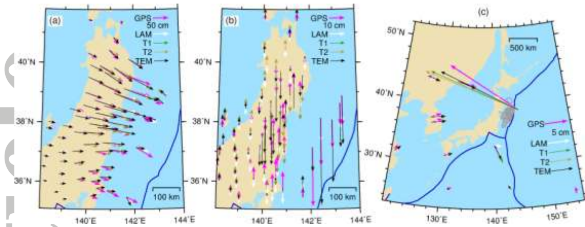
Figure 13. Comparison of two-year postseismic GPS observations at quadtree selected stations with model predicted displacements. (a) Horizontal displacements. (b) Vertical displacements. (c) Comparison of very-far-field GPS observations with model-predicted displacements. Magenta and white arrows represent GPS observations and model-predicted displacements in the LAM, respectively. Structural heterogeneities, the oceanic asthenosphere (OASP), subduction PSP (SPSP), and weakened lower crust beneath the arc (WLCA), are incorporated into the LAM step by step, that is, T1 = LAM + OASP , T2 = T1 + SPSP , and TEM = T2 + WLCA .
