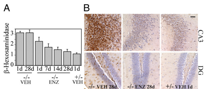
Fig. 4. Reduction of \beta -hexosaminidase and of LAMP1 after intracerebroventricular administration of NAGLU-IGFII to MPS III B mice. (A) Decrease in \beta -hexosaminidase activity (expressed in thousands of units per milligram of protein, mean \pm SD) in homogenized brain tissue from slice 1; the mouse brains are the same as were used for Fig. 2. (B) Immunohistochemical staining for LAMP1, a marker for lysosomes, in the CA3 and dentate gyrus (DG) areas of the hippocampus (slice 4), in brains removed 28 d after the last injection. (Scale bar, 50 \mu m.)
