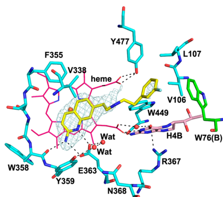
Figure 7. Active site structure of 7 bound to eNOS. The omit F_o - F_c density map for the inhibitor is shown at the 2.5 \sigma contour level. The fluorophenethyl tail of 7 shows weaker density indicative of partial disordering. Major hydrogen bonds are shown as dashed lines.
