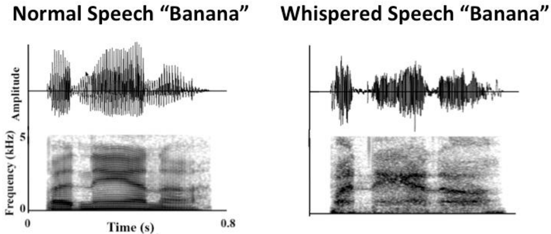
Figure 1. Waveforms (top) and narrowband spectrograms (bottom) of the word banana in different acoustic forms: a) normal speech, and b) whispered speech.
